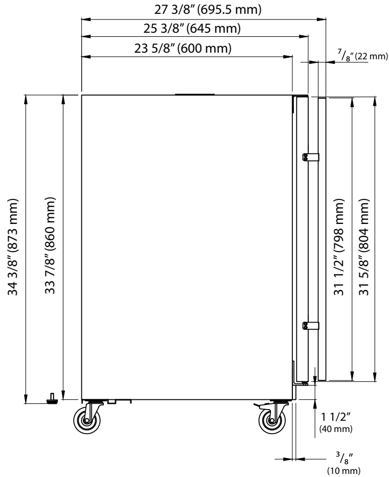
Side View
