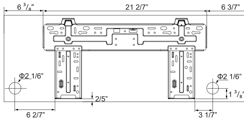
Wall Mounting Frame
