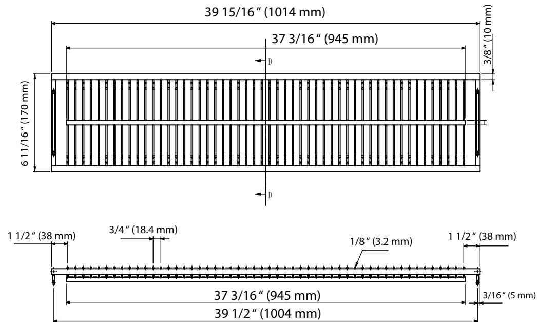
Warming Rack
