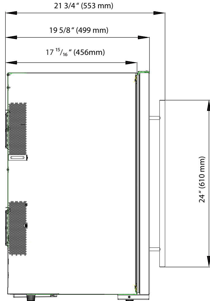
Side View
