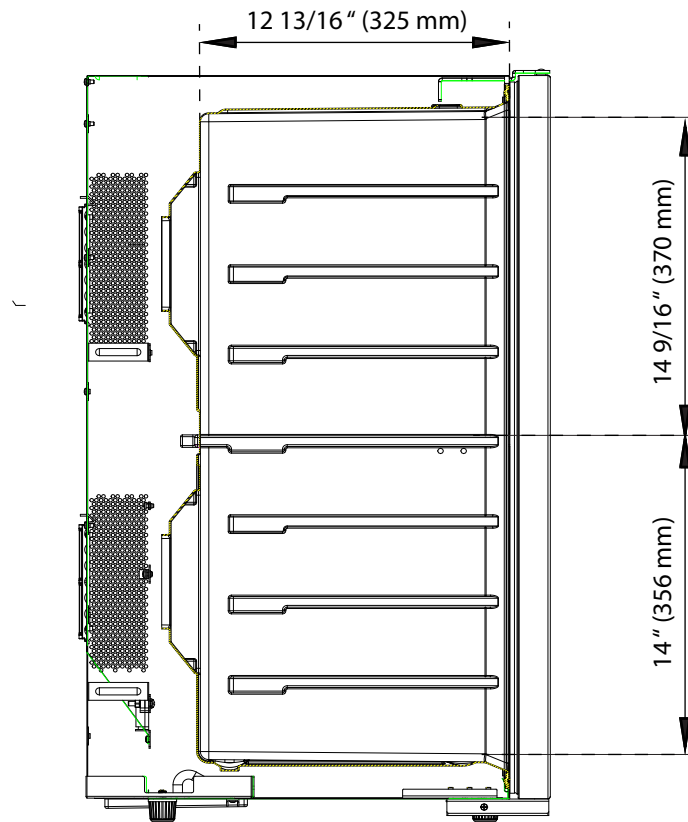
Side View
