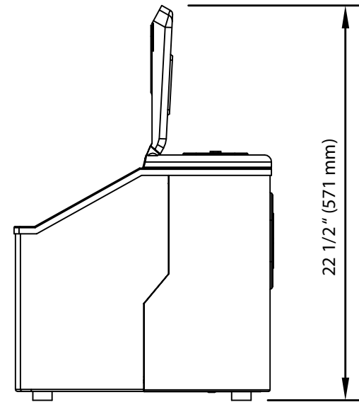
Door Swing View
