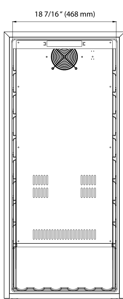
Front View
