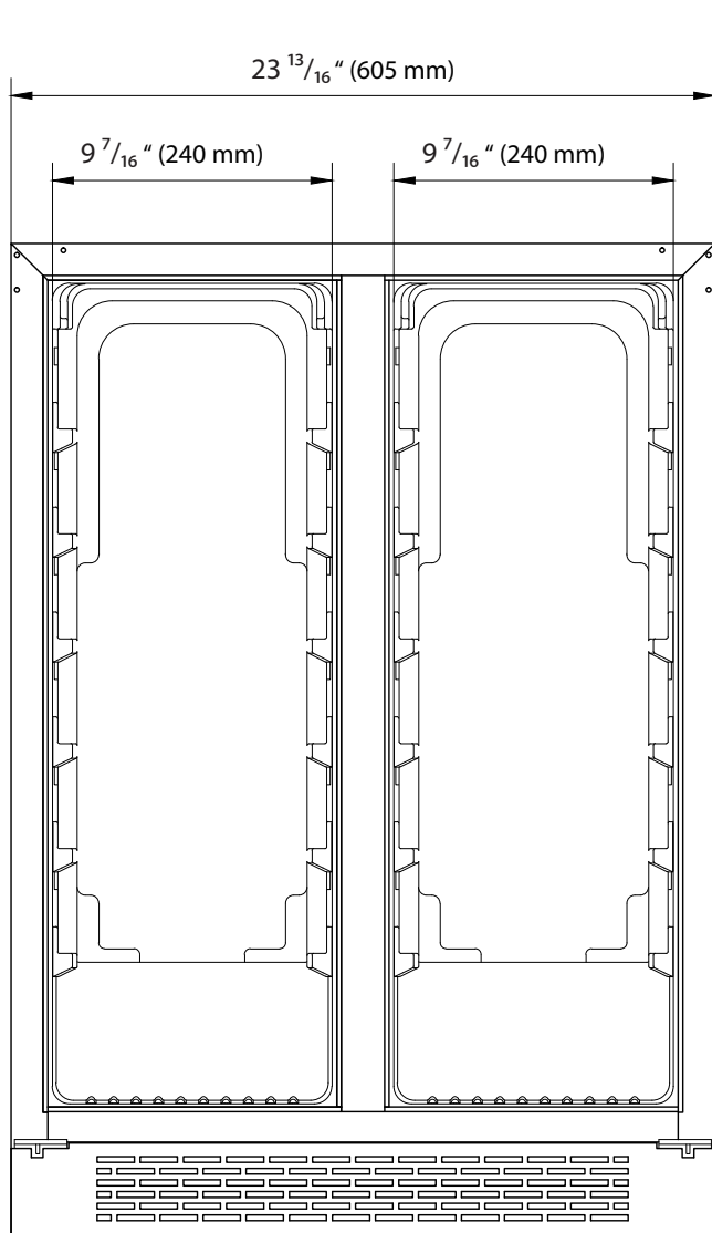
Front View
