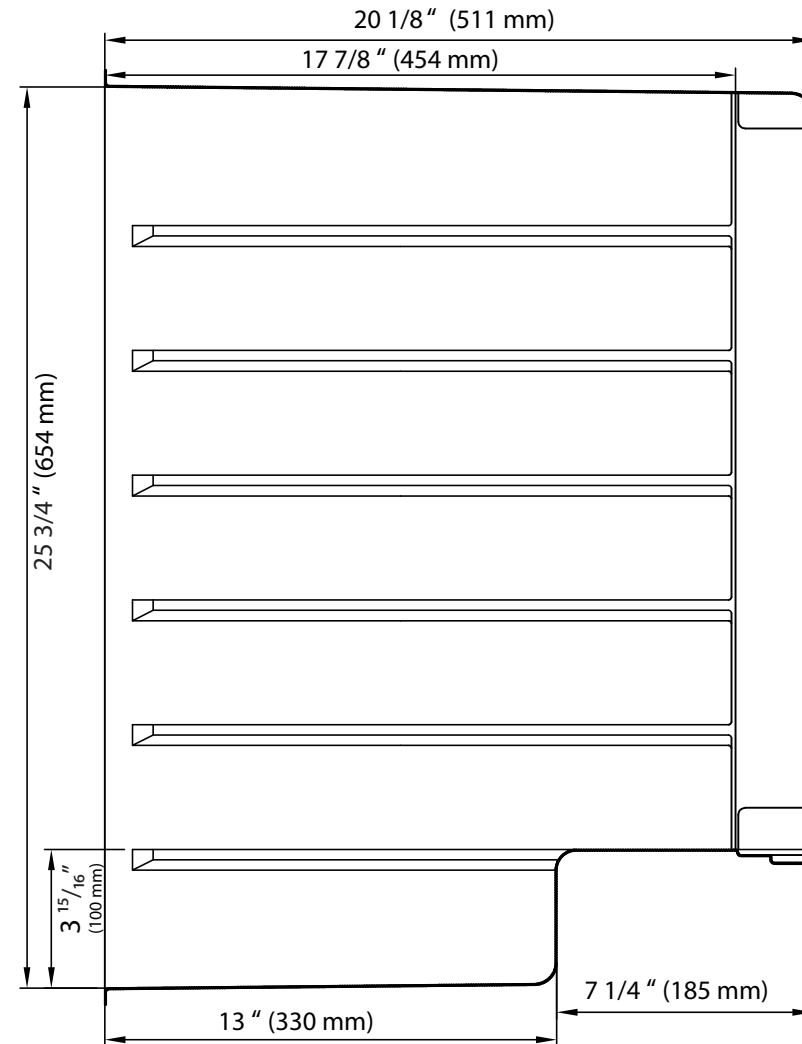
Side View
