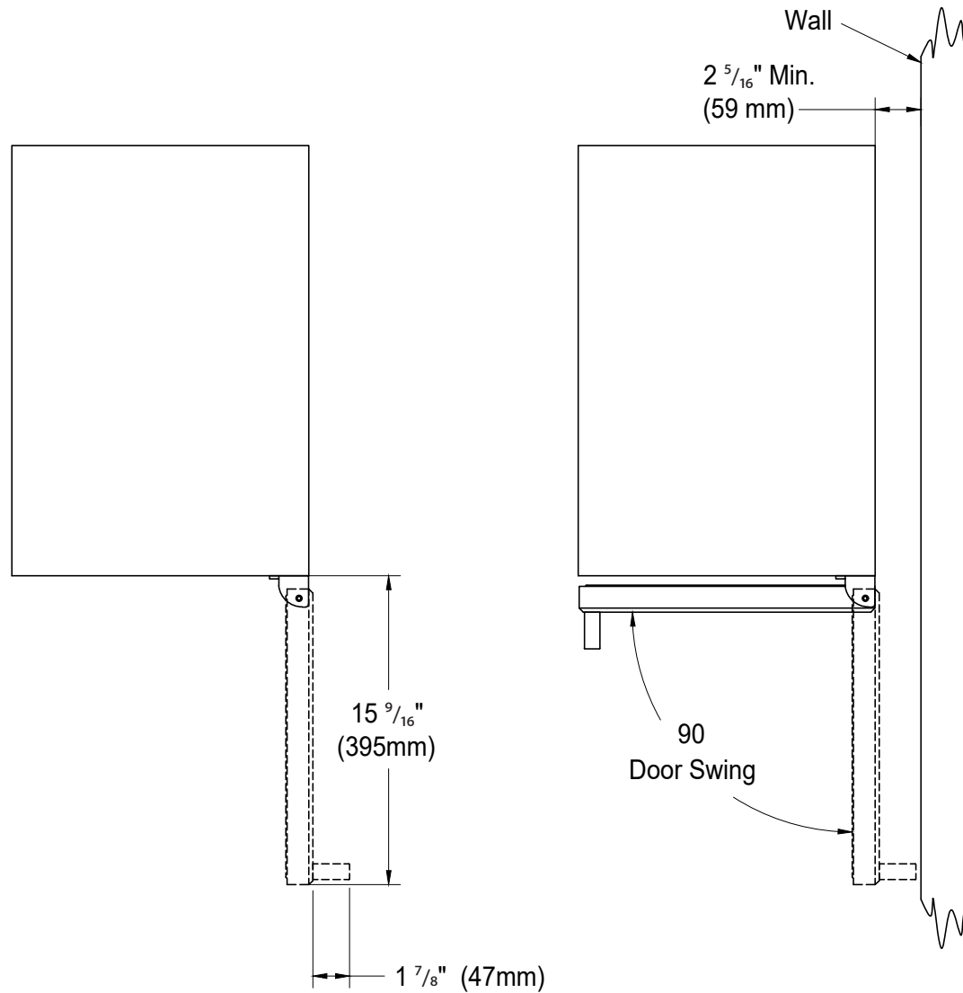
Top View
