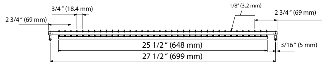
Warming Rack
